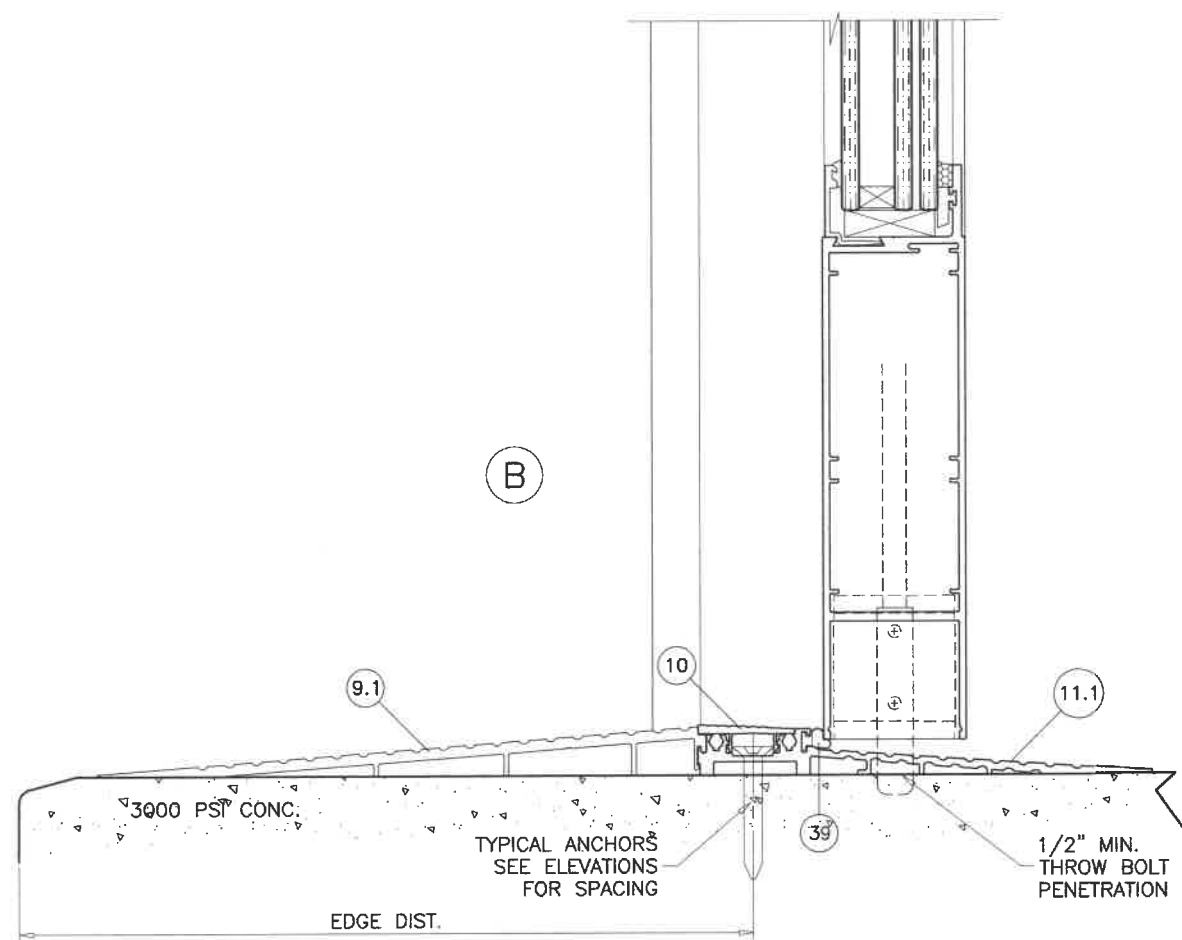
ADA COMPLIANT THRESHOLD
