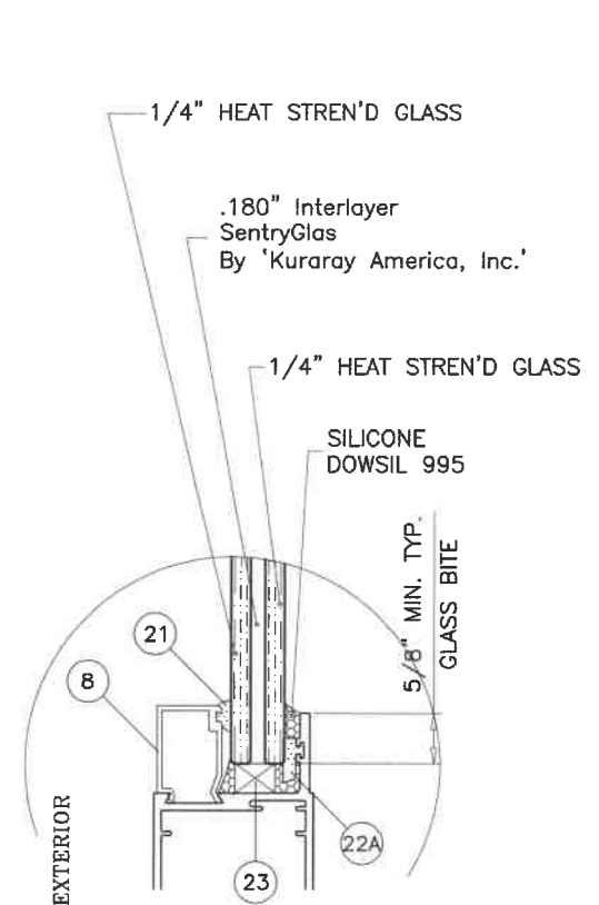
GLASS TYPE 'B'
